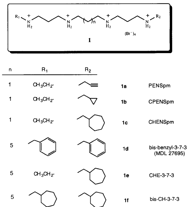
Figure 1. Bis(alkyl)-substituted polyamine analogues.
